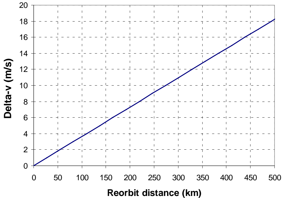
Figure 5 \Delta V requirements as a function of re-orbit distance above GEO
