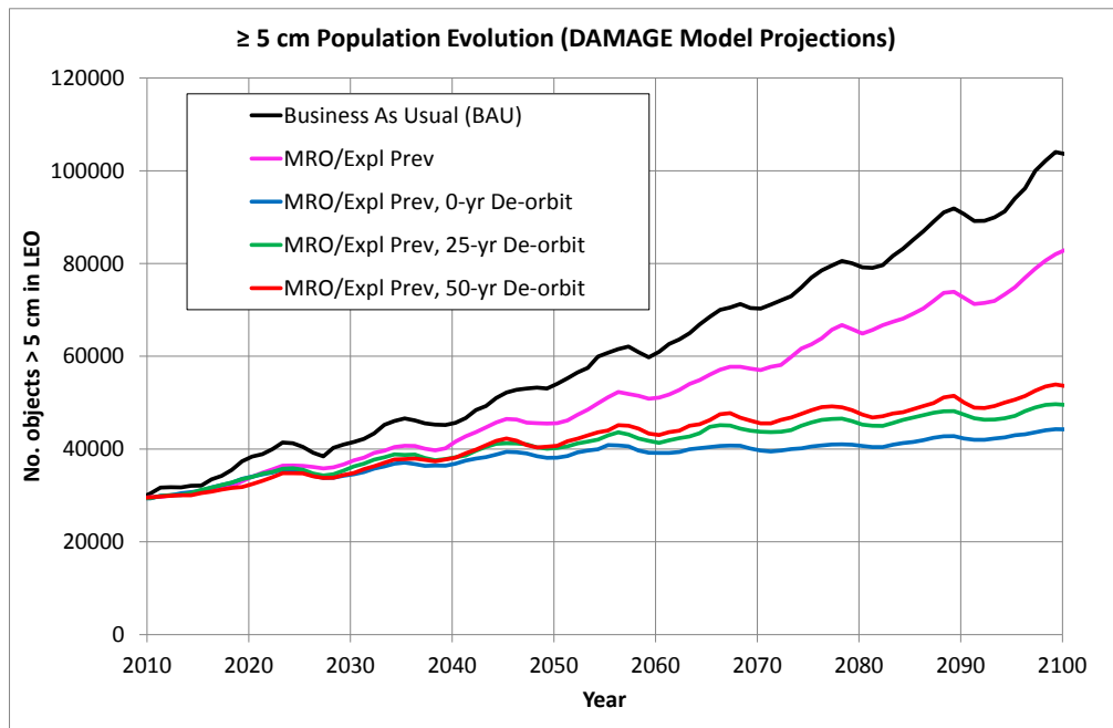
Figure 6 Debris (≥ 5 cm) Average Population Evolution from DAMAGE
