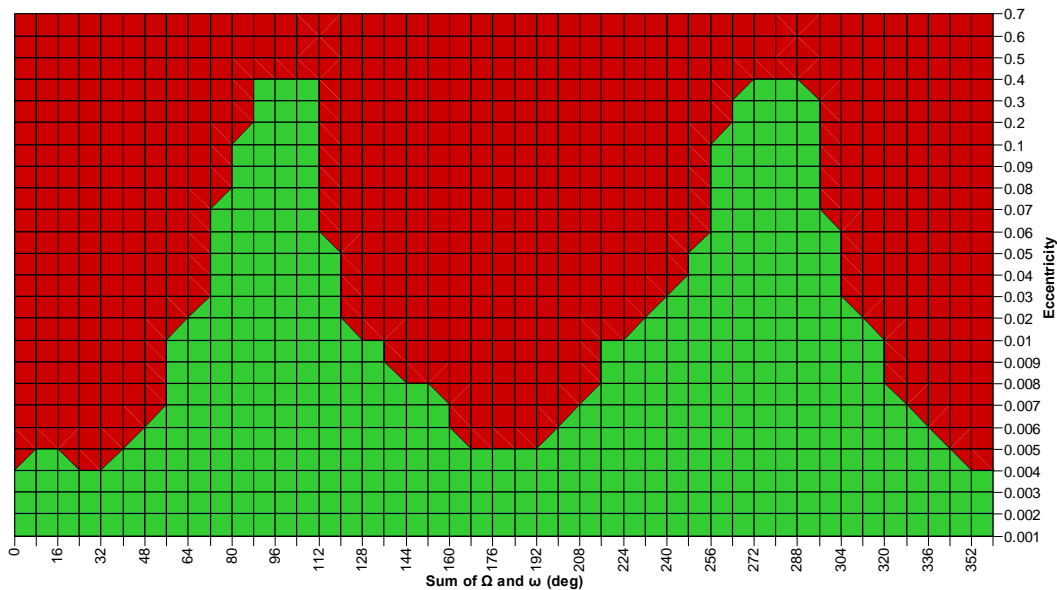
Figure 4 Example combinations of \Omega and \omega that will cause an orbit to re-enter the GEO protected region over 40 years.
