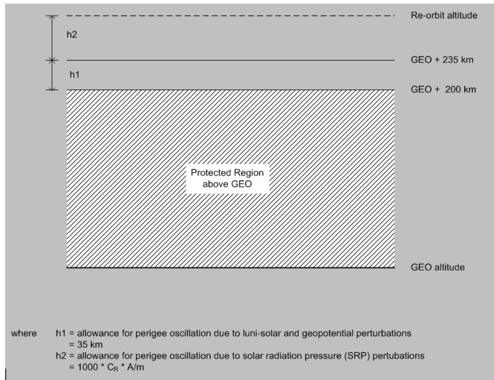
Figure 3 Schematic showing the basis for the formula describing the recommended minimum increase in perigee altitude
